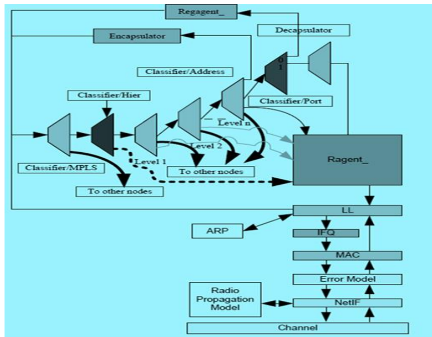
Fig.2. Radio propagation system
