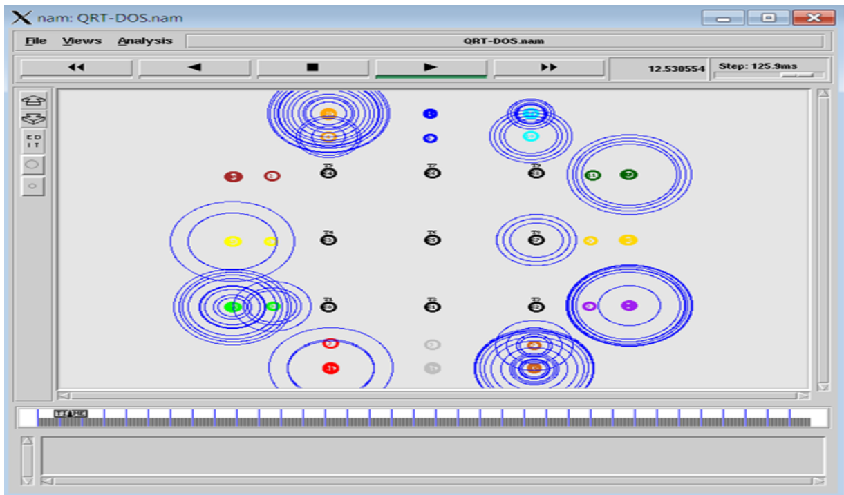
Fig.4. QRT-DOS Prevention Scenario
