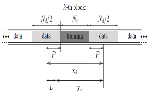
Fig. 1. Partitioning of the transmitted symbol vectors into blocks, each consisting of N_t training and N_d data symbol vectors.
