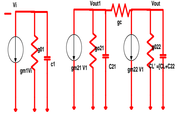
Fig. 2: small signal model
