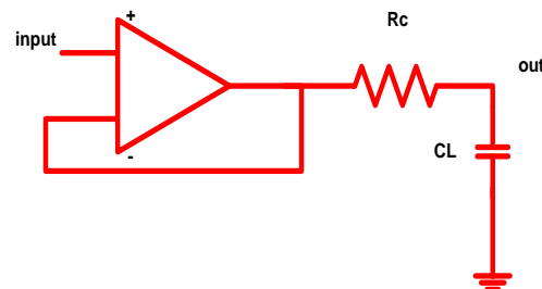
Fig. 1: zero compensation buffer amplifiers
