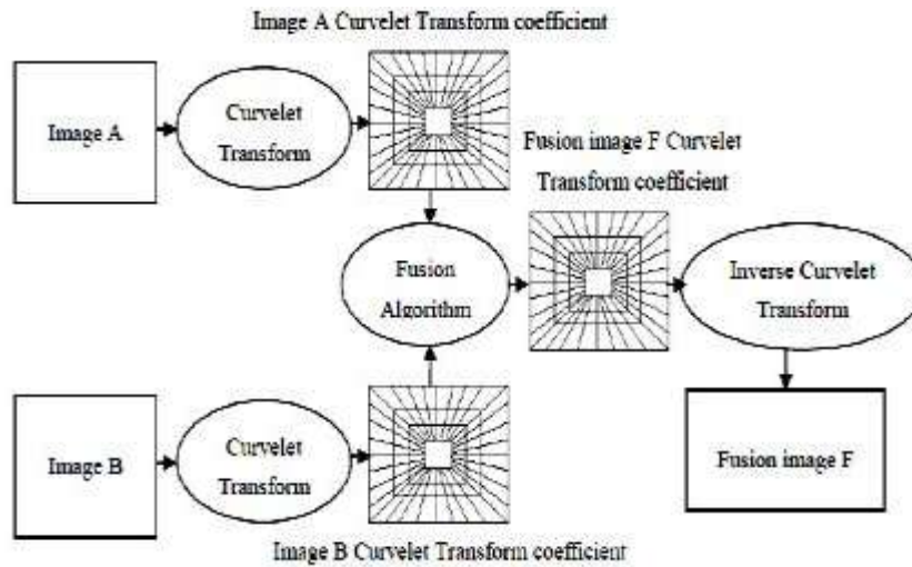
Fig 1: Process of image fusion algorithm base on Curvelet transform.
